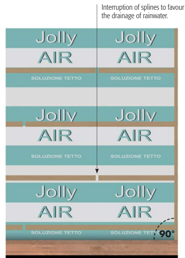
The gutter line must be perfectly perpendicular (with an angle of 90°) to the lateral ridge.
